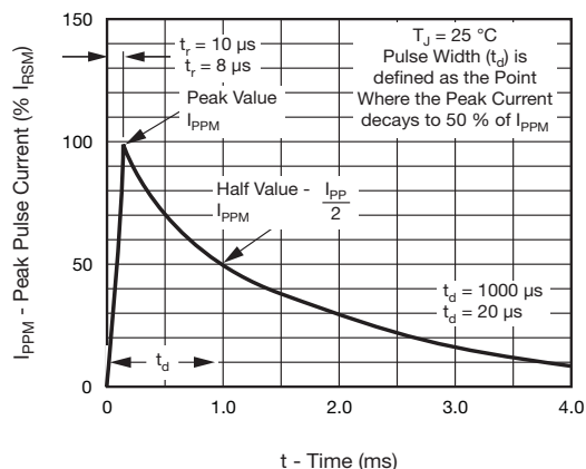
Fig. 1 - Pulse Waveform
