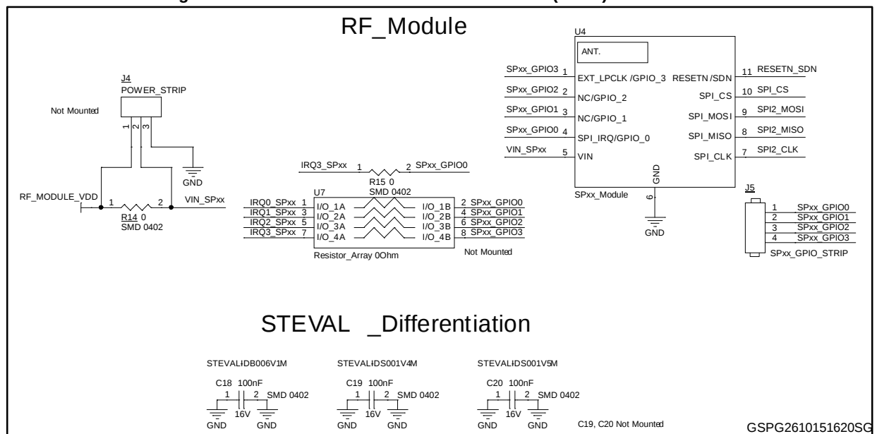
Figure 4: STEVAL-IDB006V1M circuit schematic (4 of 4)
