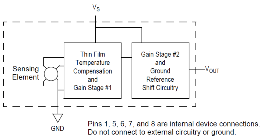
Figure 1. Fully integrated pressure sensor schematic
