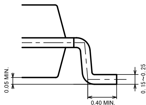
Details of "F" part
