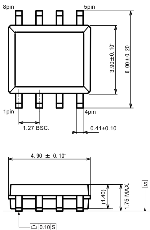
8-pin plastic SOP
