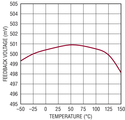
Feedback Voltage
