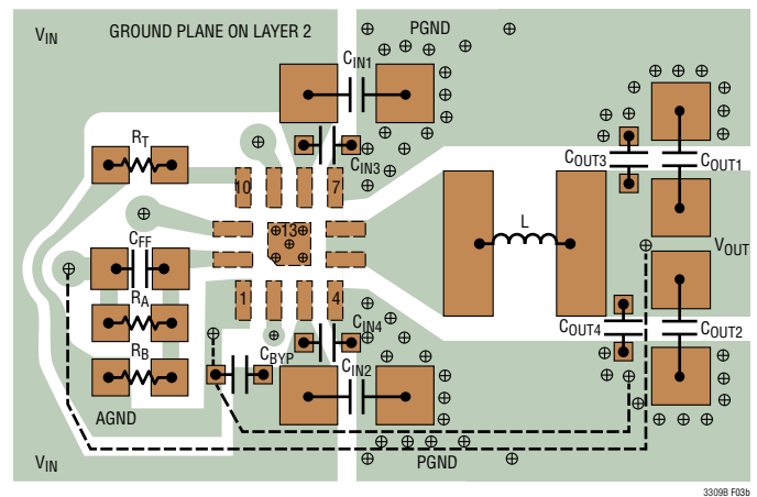
(3b) Recommended PCB Layout for the LTC3309B with Capacitors C_{OUT1} and C_{OUT2} Rotated by 90°, which Reduces High-Frequency Output Ripple. Optional 0201 Capacitors C_{OUT3} and C_{OUT4} Further Improve The High-Frequency Output Ripple. Five 5mil Vias Are Used within the EPAD. For Layouts where 5mil Vias Are Not Allowed, It Is Recommended to Use Either Four 8mil Vias or a Single (Filled or Tented) 12mil Diameter Via
