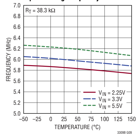
R_T Switching Frequency
