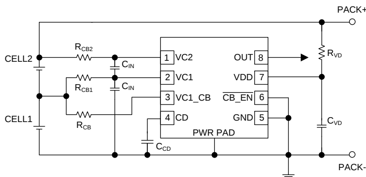
Simplified Schematic
