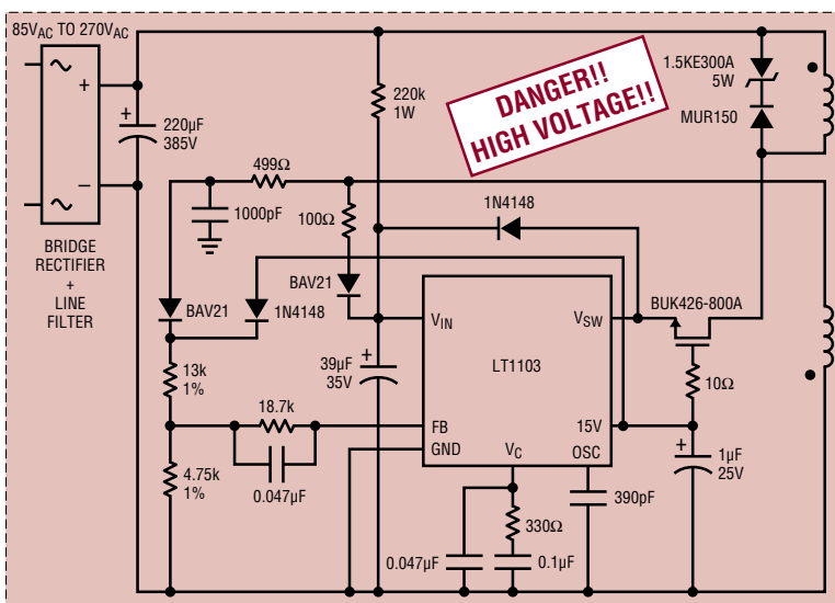
Fully Isolated Flyback 100kHz 50W Converter with Load Regulation Compensation
