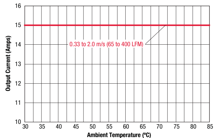
Maximum Current Temperature Derating at Sea Level (VIN = 36 and VOUT = 48V, airflow is from pin 3 to pin 1)
