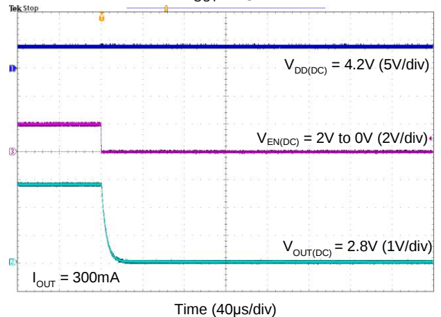
Enable Turn-Off Response V OUT =2.8V
