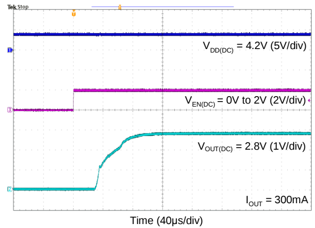
Enable Turn-On Response V OUT =2.8V
