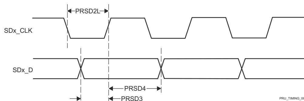
Figure 6-95. PRU_ICSSG PRU SD_CLK Rising Active Edge
