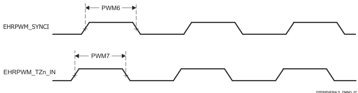
Figure 6-31. EPWM Timing Requirements
