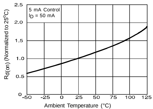
Figure 4. Typical On-Resistance
