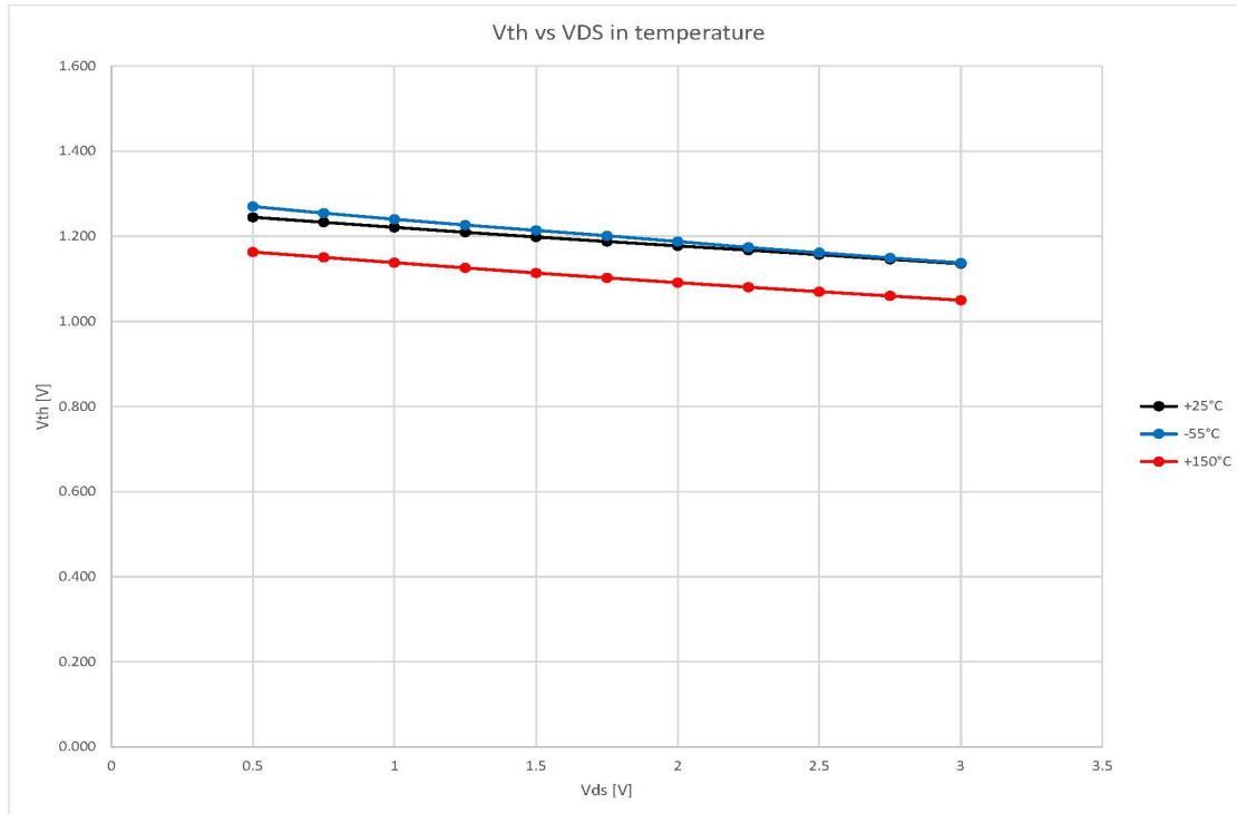
Figure 18: V TH vs V DS
