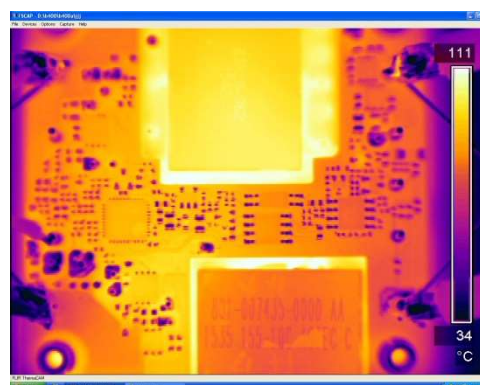
Figure 14 Infrared thermal image, 48Vin @ full load, 200LFM, 25°C
