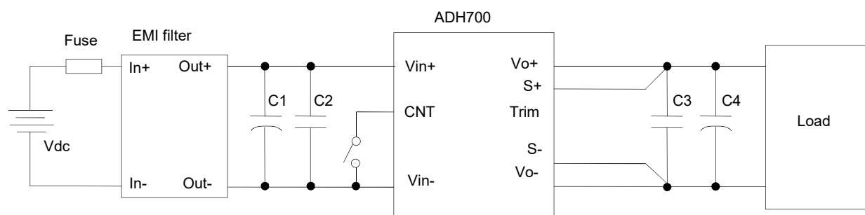
Figure 15 Typical application
