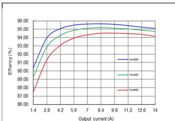
Figure 9: ADH700-48S50-6L Efficiency Curves @ 25 °C, 400LFM, Vo=50V
