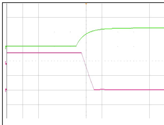
Figure 6: ADH700-48S50-6L Output voltage shutdown by remote OFF (2mS/div) Ch 2: Remote ON (5V/div) Ch 2: Vo (20V/div)
