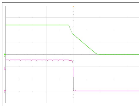
Figure 4: ADH700-48S50-6L Output voltage shut down by power Off (50ms/div) Ch 2: Vin (20V/div) Ch 4: Vo (10V/div)
