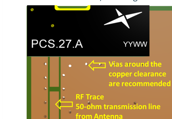
PCS.27.A antenna mounted on a PCB, showing transmission line and integration notes.
