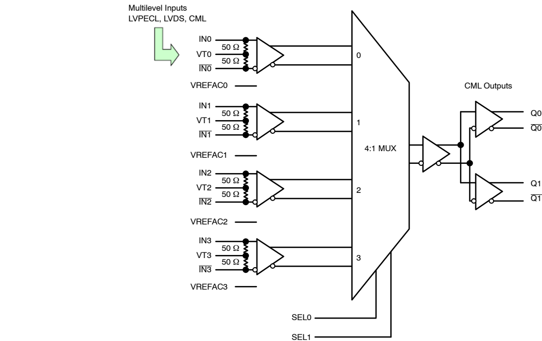
Figure 1. Simplified Block Diagram
