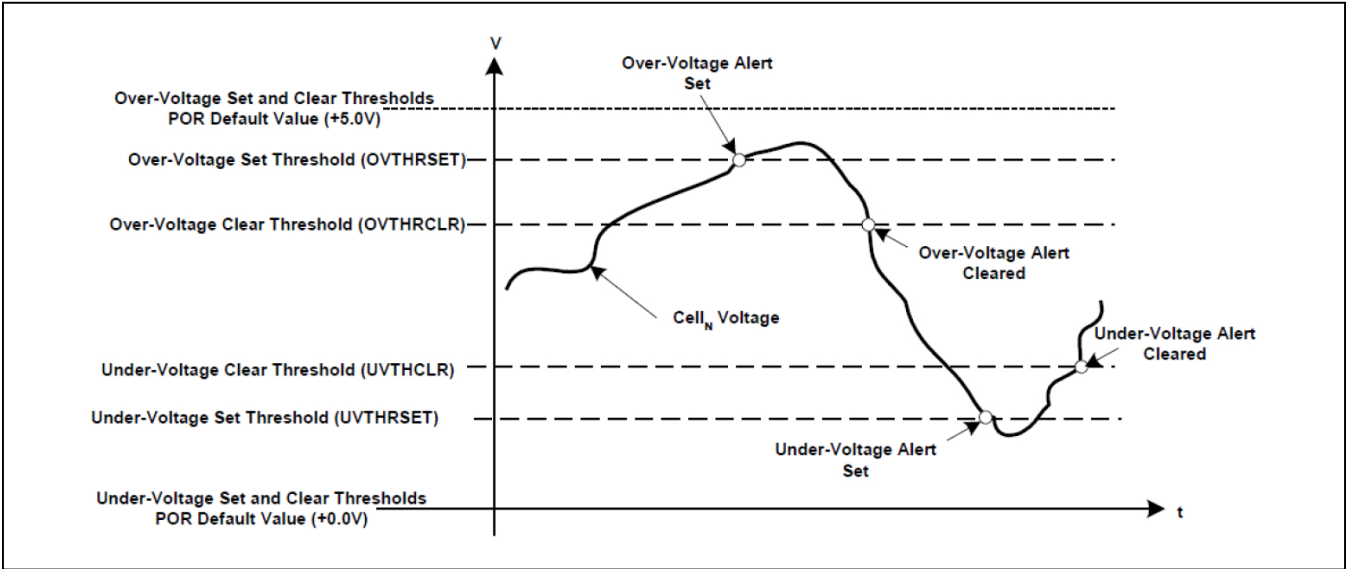
Figure 14. Programmable Overvoltage and Undervoltage Thresholds Diagram
