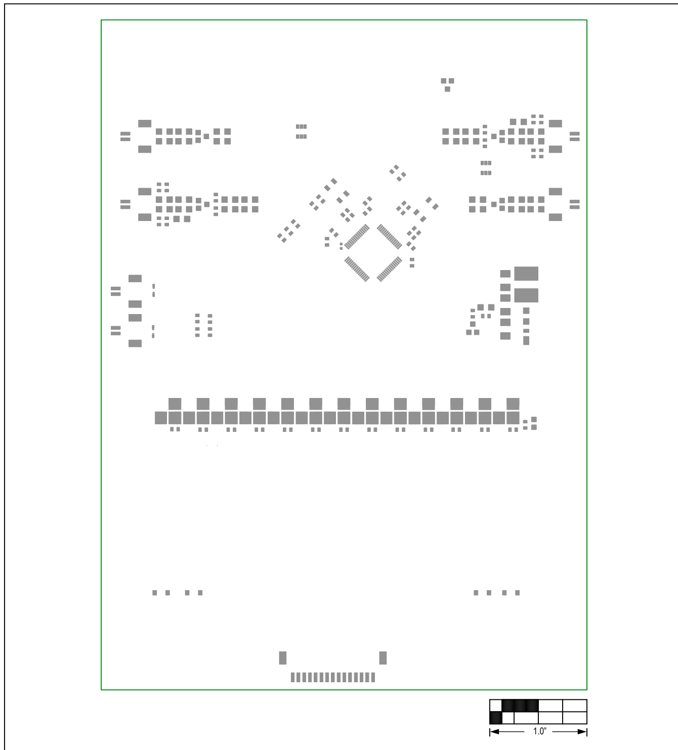
MAX17843 EV Kit PCB Layout—Top Pastemask
