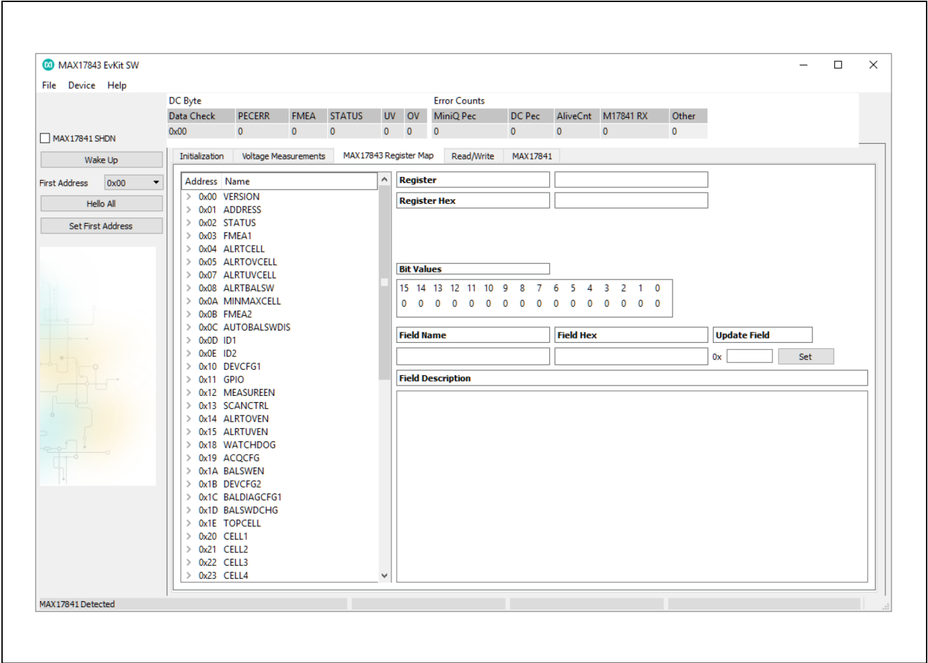
Figure 4. MAX17843 EV Kit Software (MAX17843 Register Map Tab)
