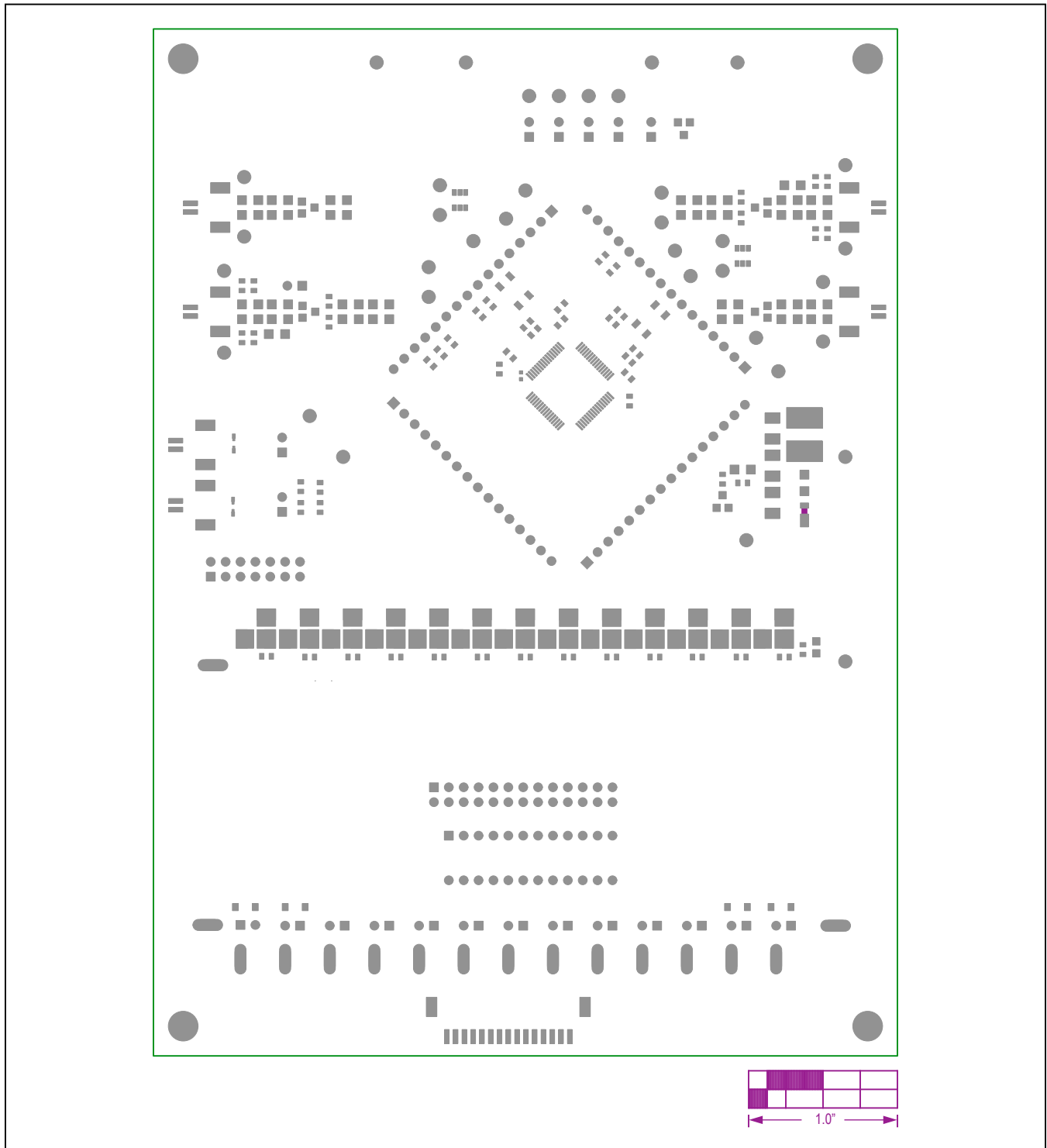
MAX17843 EV Kit PCB Layout—Top Soldermask
