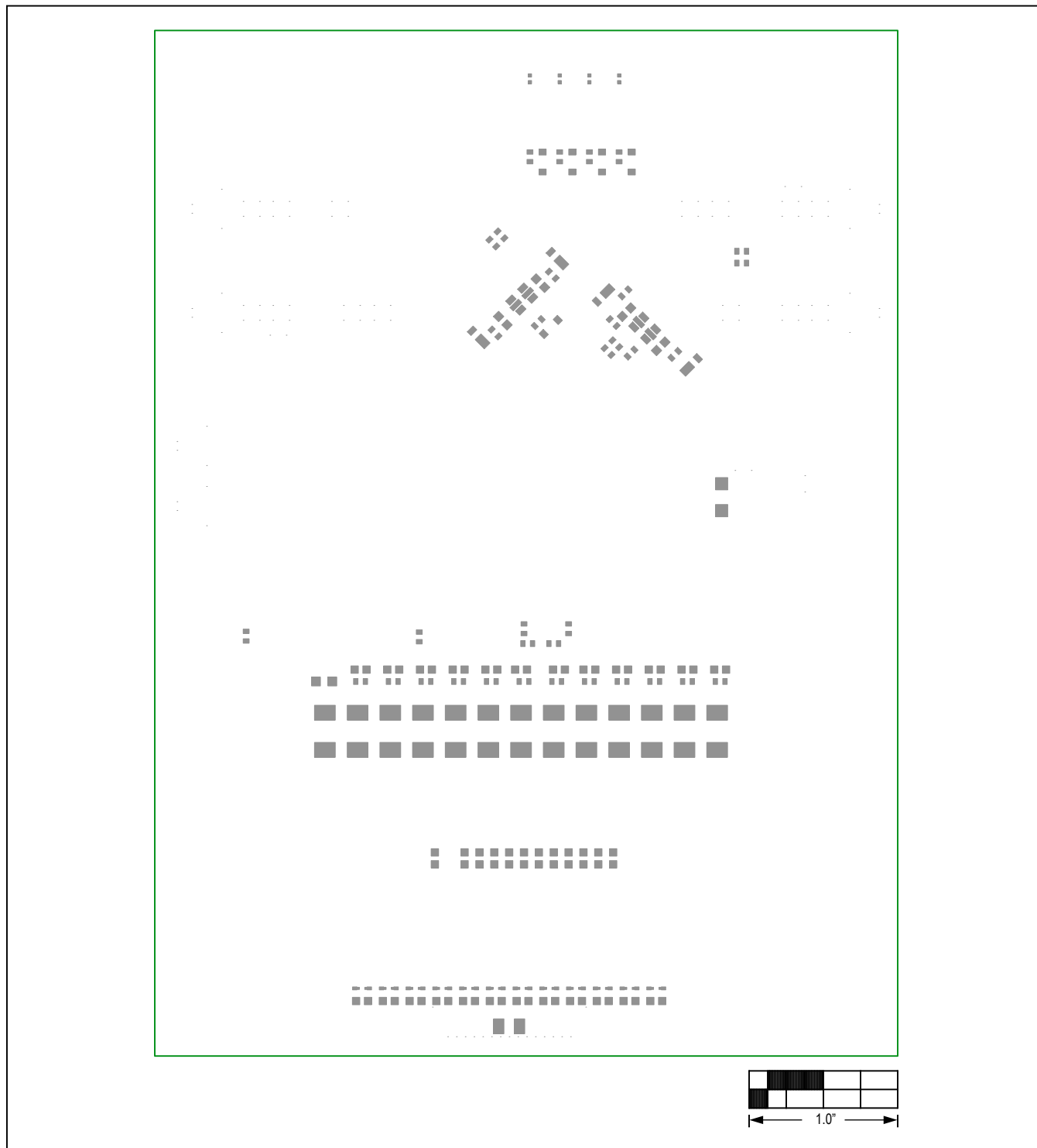
MAX17843 EV Kit PCB Layout—Bottom Pastemask
