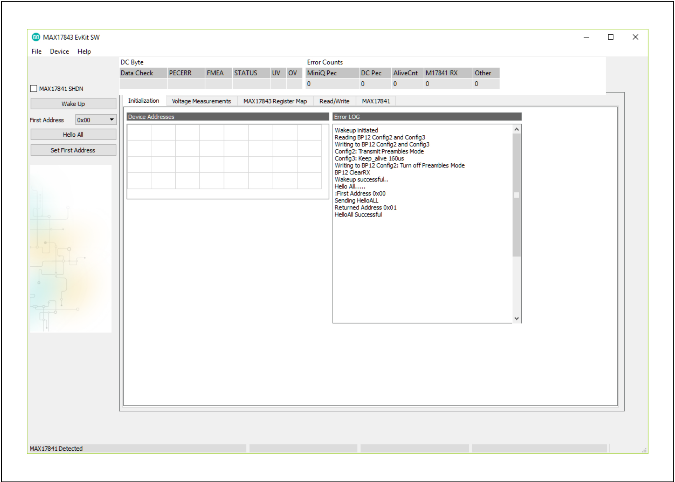
Figure 2. MAX17843 EV Kit Software (Installation Tab—Wake Up and Hello All)
