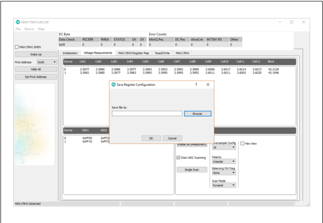
Figure 13. MAX17843 Evaluation Kit Software (Voltage Measurements Tab—Save Register Configuration Dialog Box)
