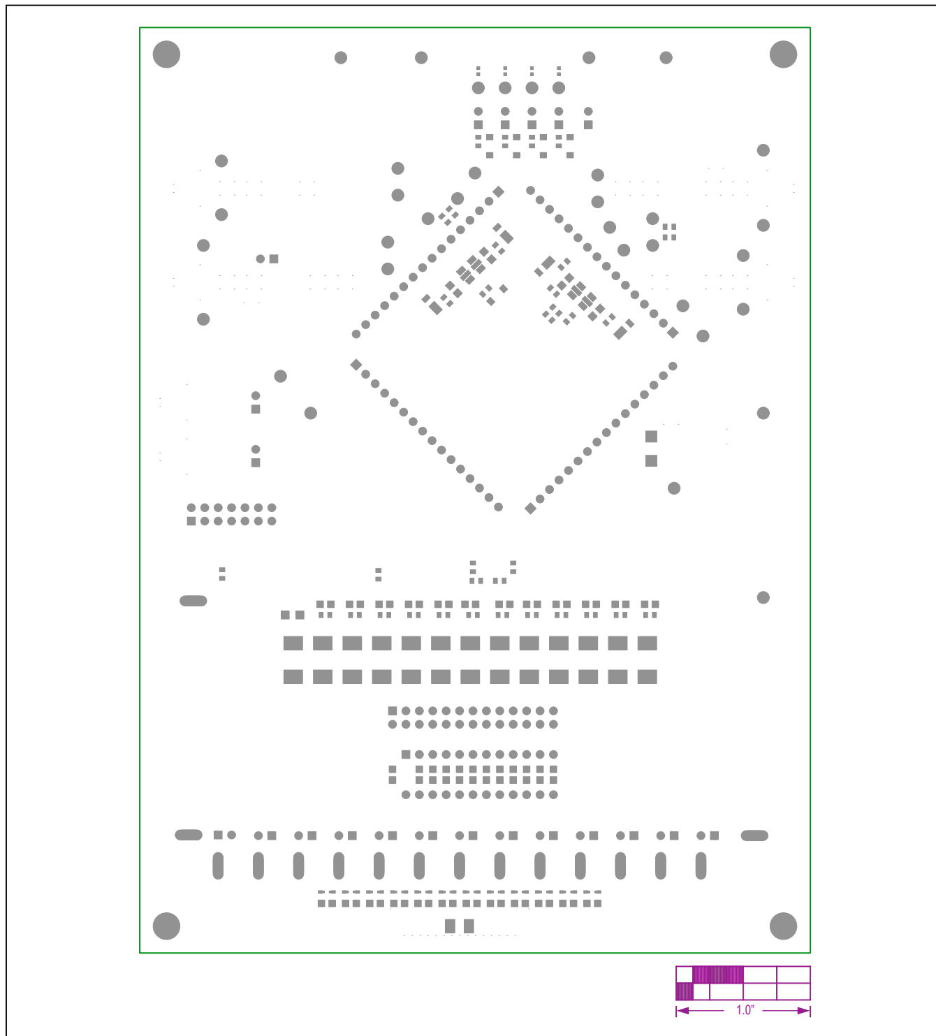
MAX17843 EV Kit PCB Layout—Bottom Soldermask
