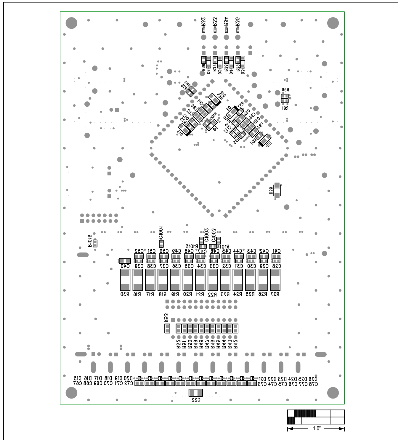
MAX17843 EV Kit Component Placement Guide—Bottom Silkscreen
