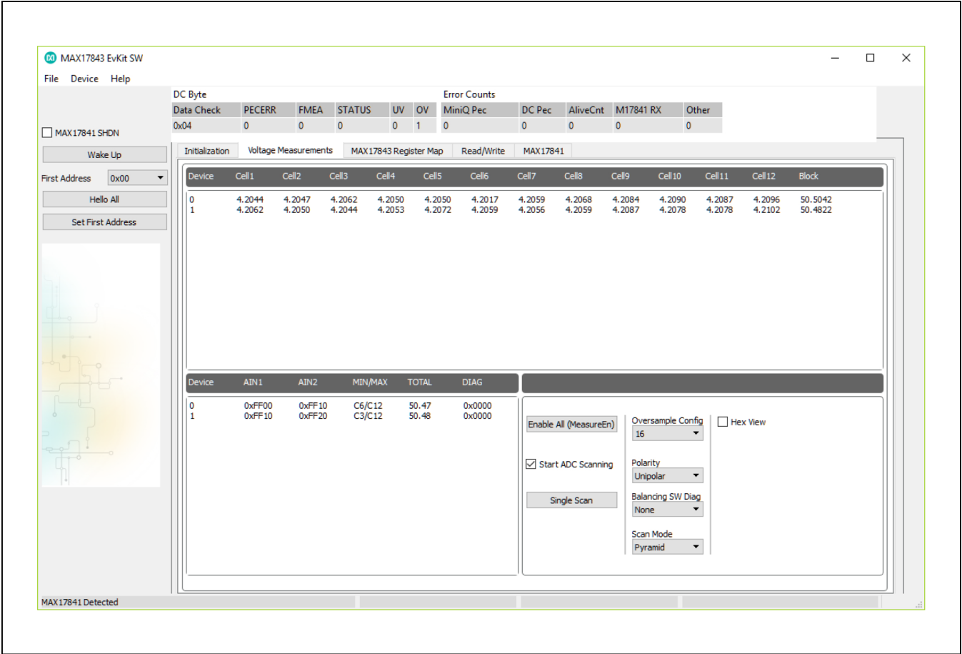
Figure 15. MAX17843 Evaluation Kit Software (Voltage Measurements Tab—OV Flag)
