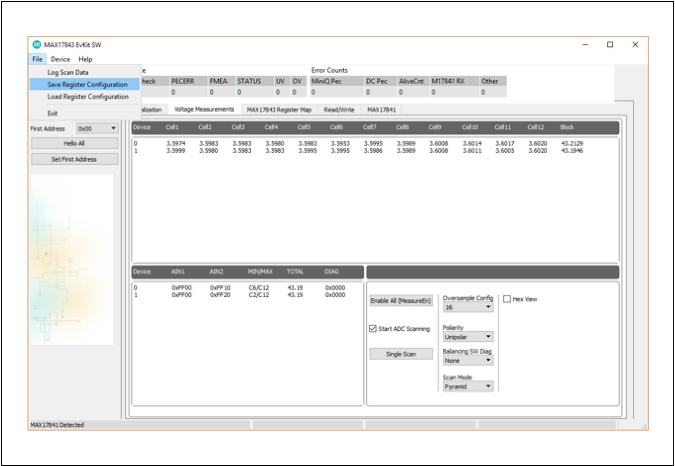
Figure 12. MAX17843 Evaluation Kit Software (Voltage Measurements Tab—Save/Load Register Configuration)
