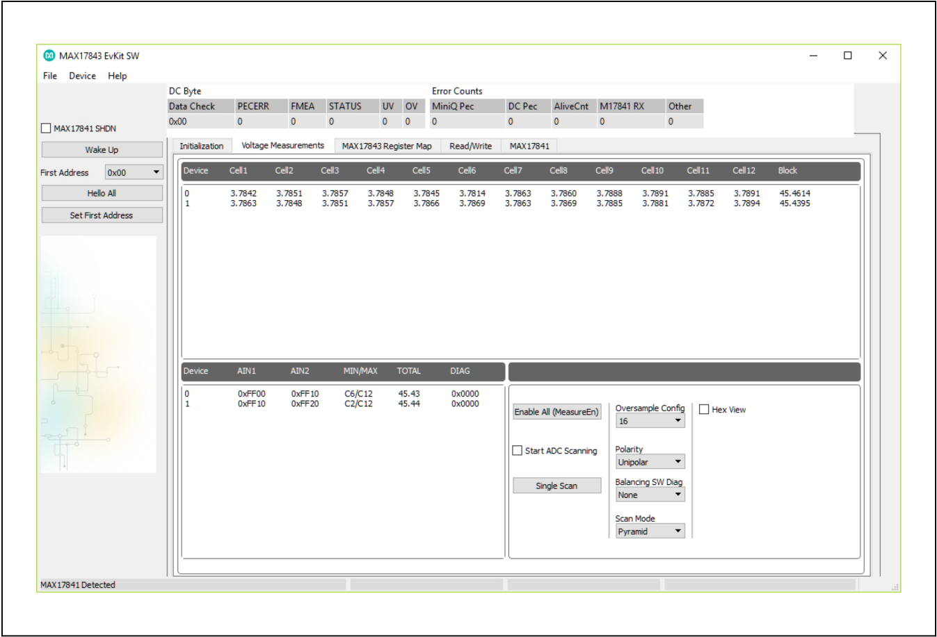
Figure 16. MAX17843 Evaluation Kit Software (Voltage Measurements Tab—OV Flag Cleared)
