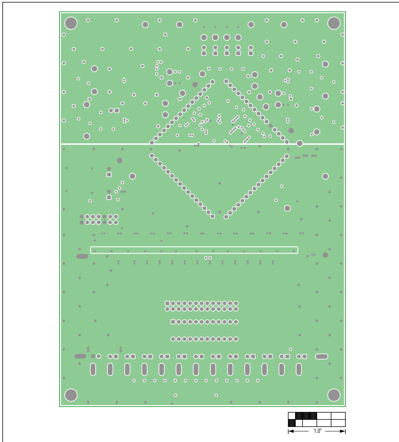
MAX17843 EV Kit PCB Layout—Layer 3 (PWR)
