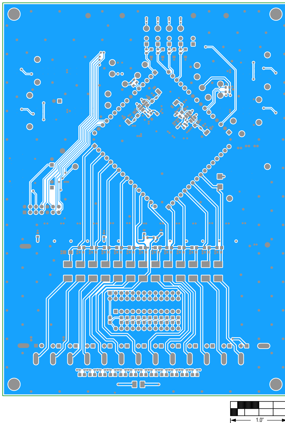
MAX17843 EV Kit PCB Layout—Solder Side
