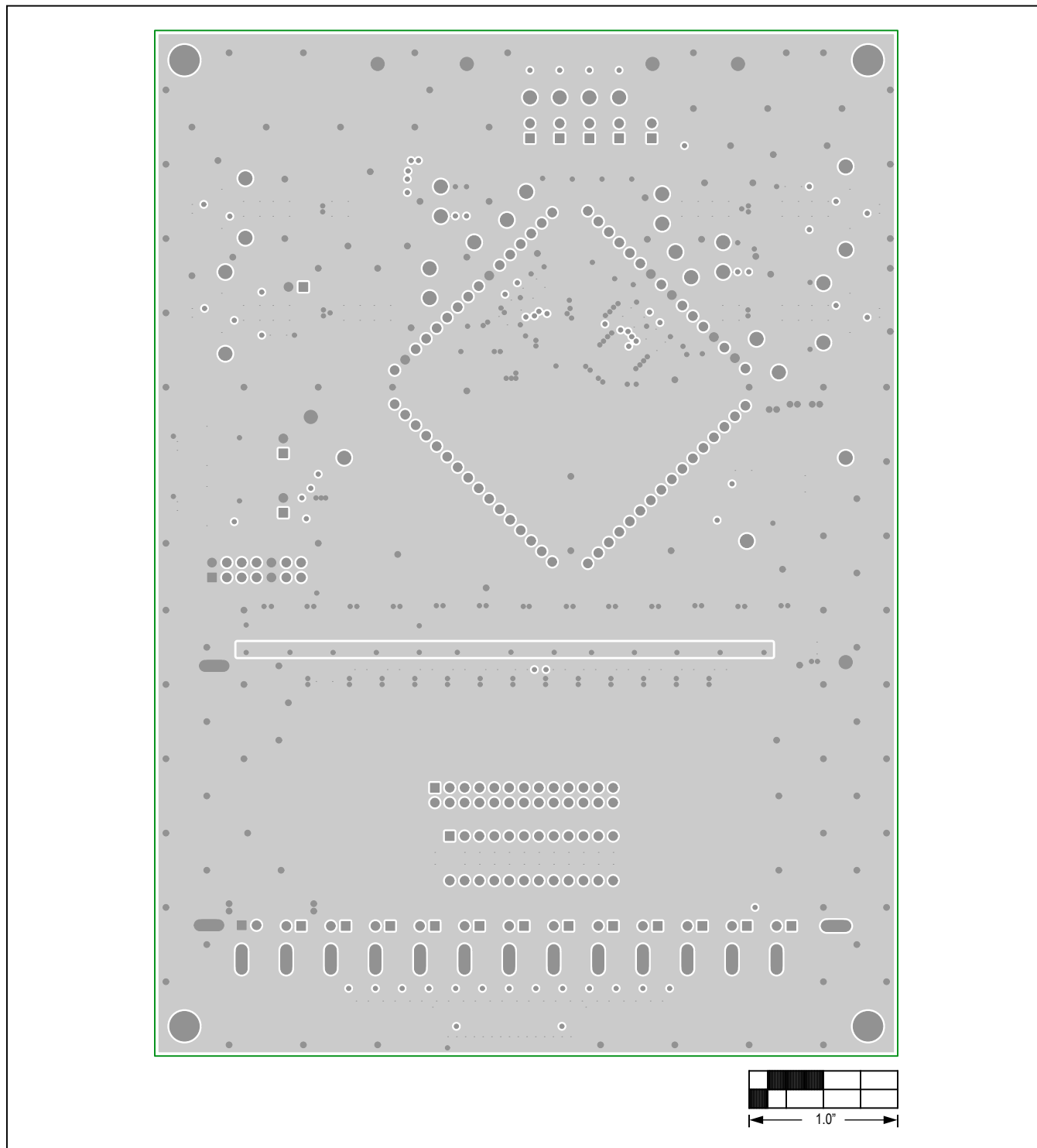
MAX17843 EV Kit PCB Layout—Layer 2 (GND)
