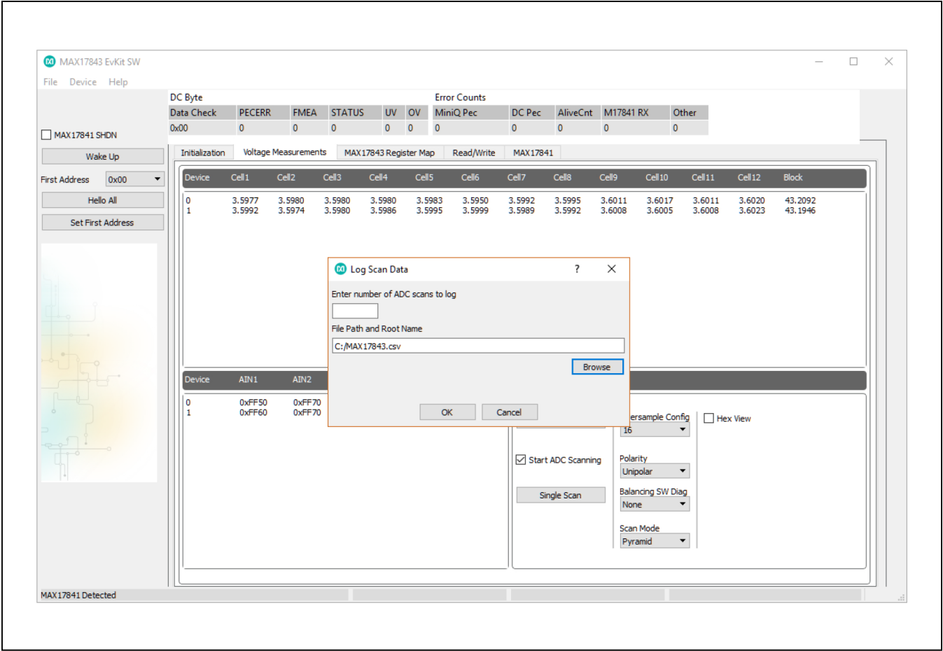
Figure 11. MAX17843 Evaluation Kit Software (Voltage Measurements Tab—Enter Number of Scans and Choose File Path Dialog Box)
