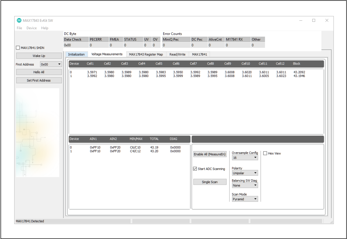
Figure 9. MAX17843 Evaluation Kit Software (Voltage Measurements Tab—Start ADC Scanning)
