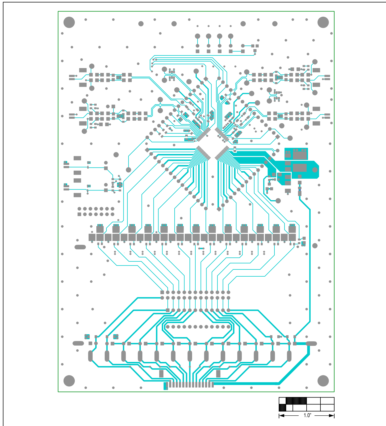
MAX17843 EV Kit PCB Layout—Component Side
