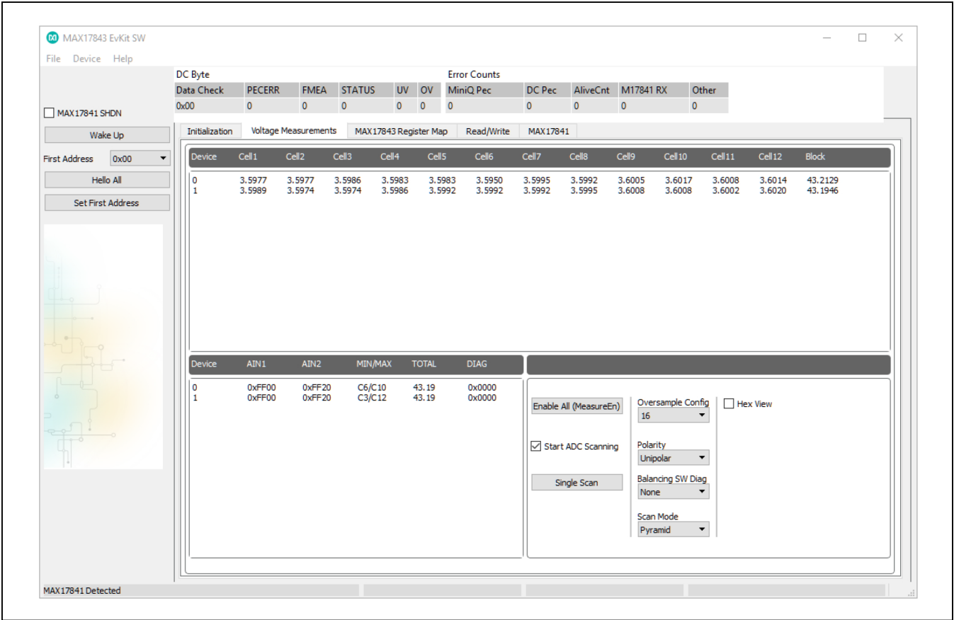
Figure 7. MAX17843 Evaluation Kit Software (Voltage Measurements Tab)
