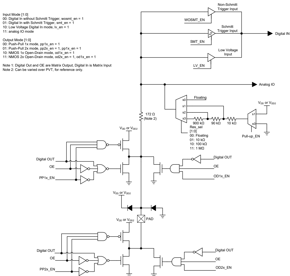
Figure 4: Matrix OE IO Structure Diagram
