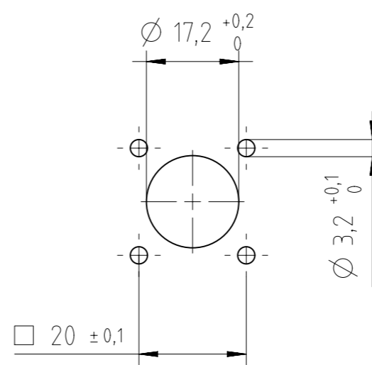
Panel Cutout M1:1
