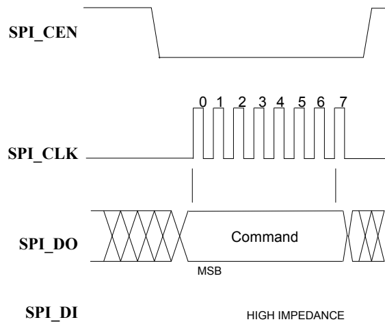
Figure 5.8 SPI Command Only Sequence
