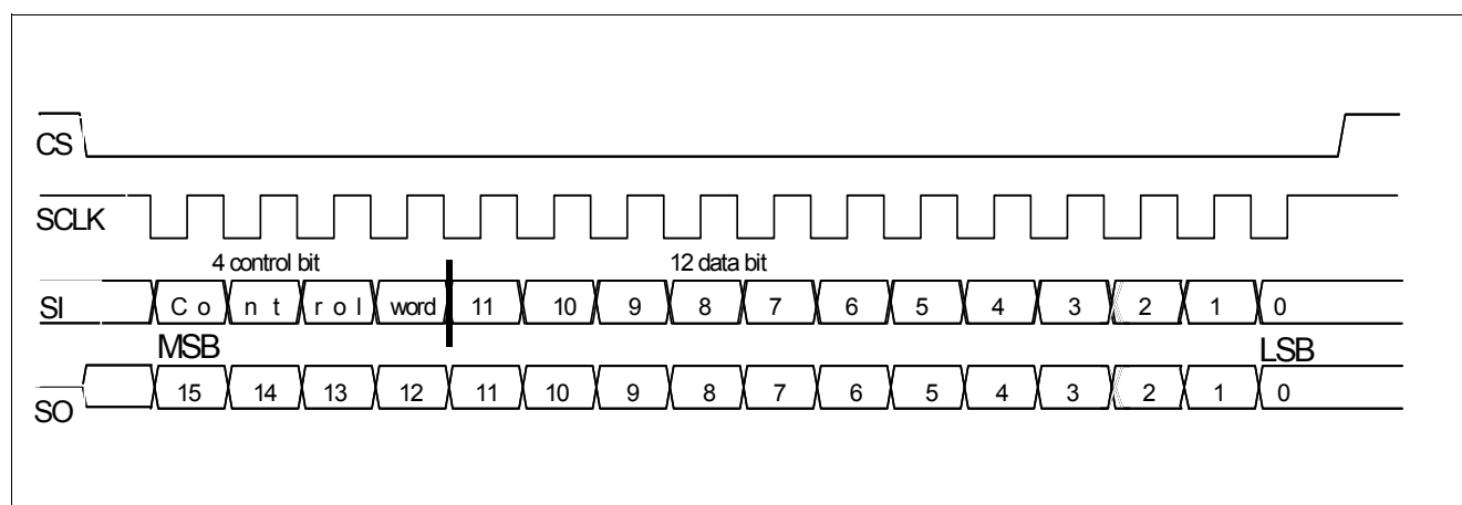
Figure 13 Serial Interface
