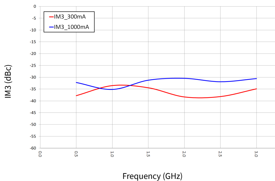
Figure 7 - IM3 vs. Frequency of the CG2H30070F as Measured in the Single-ended Demonstration Amplifier CG2H30070F-AMP P_{OUT} = 40 dBm, Temperature = 25°C
