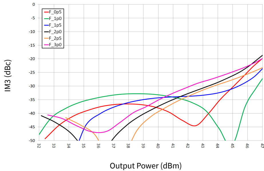
Figure 5 - IM3 vs. Output Power of the CG2H30070F as Measured in the Single-ended Demonstration Amplifier CG2H30070F-AMP I_{DQ} = 300 mA, Temperature = 25°C
