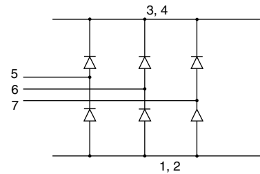
Electrical circuit
