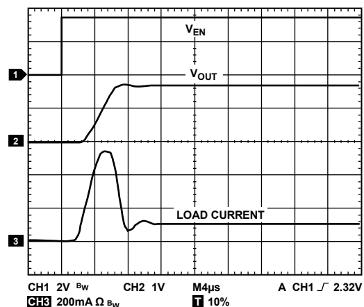
Figure 28. Typical Rise Time and Inrush Current, C_{LOAD} = 1\text{ }\mu\text{F} , V_{IN} = 1.8\text{ V} , Load = 200\text{ mA}
