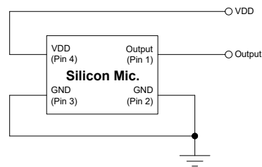
Figure 3. SMO04C-38 Interface Schematic Diagram
