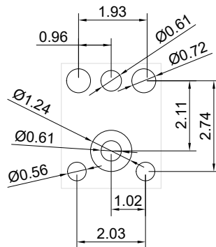
Figure 9. PCB solder pad layout for SMO04C-38
