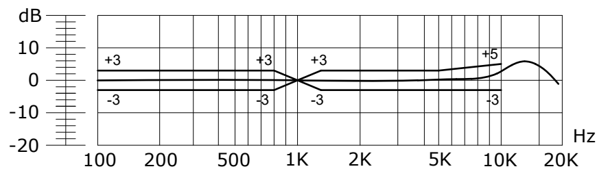
Figure 5. Frequency Response
