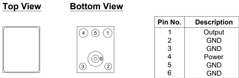
Figure 4. Electrical Layout of SMO04C-38
