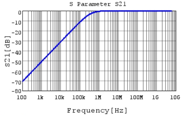
GRM033R71A472KA01 S21 DC0V, 25degC
