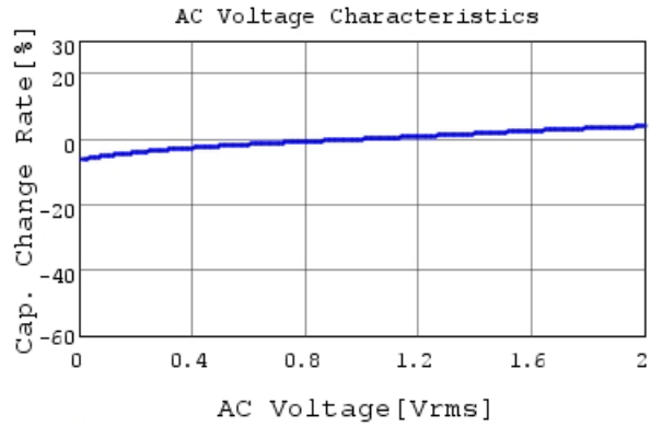
GRM033R71A472KA01 C-AC Voltage capchange, Dc
