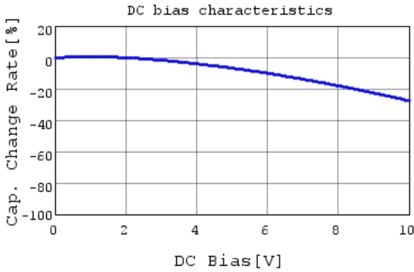
GRM033R71A472KA01 C-DC bias capchange, 25.0c
