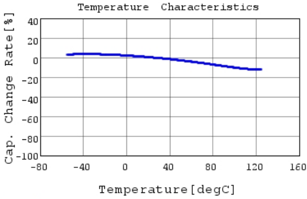
GRM033R71A472KA01 C-Temp. capchange, DC0.0V,
