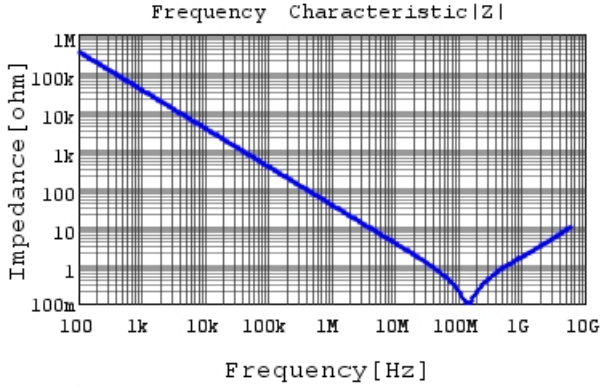
GRM033R71A472KA01 |Z| DCOV, 25degC
