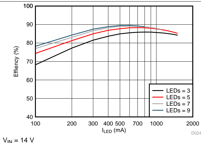
Figure 44. Efficiency from 100 mA to 1.5 A
