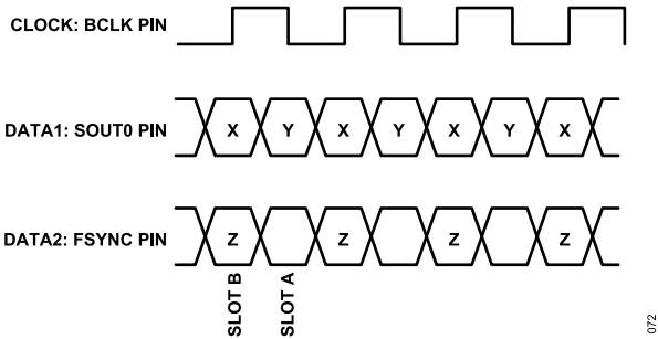
Figure 72. Example PDM Port Data Format
