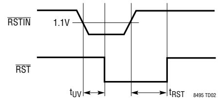
\overline{RSTIN} Timing
