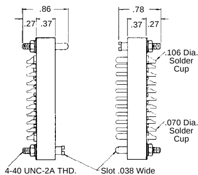
Plug MRA 50-8P-G
