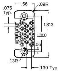
18 Contacts XMRE 18
