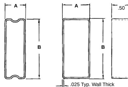
Potting form plan view for 9 to 26 contacts
