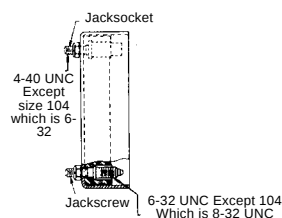
Connector with fixed Jackscrews Code designation: F
