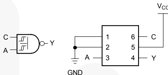
Figure 4. 2-Input NAND Gate
