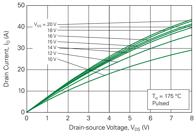
Fig. 3. Typical Output Characteristics @ T_{vj} = 175\text{ }^{\circ}\text{C}
