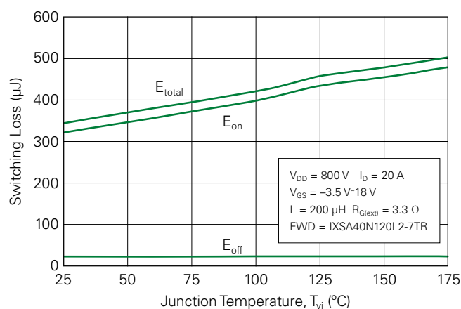
Fig. 22. Switching Energy vs. Temperature
