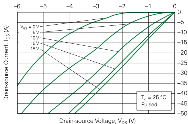
Fig. 14. 3 rd Quadrant Curves @ T_{vj} = 25\text{ }^{\circ}\text{C}
