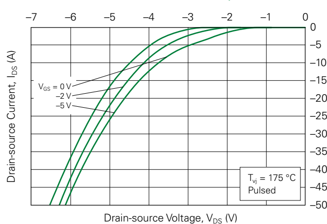
Fig. 12. Body Diode Curves @ T_{vj} = 175 °C
