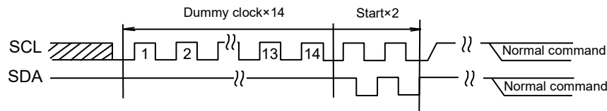
Figure 40-(a). The Case of Dummy Clock×14 + START×2 + Command Input
