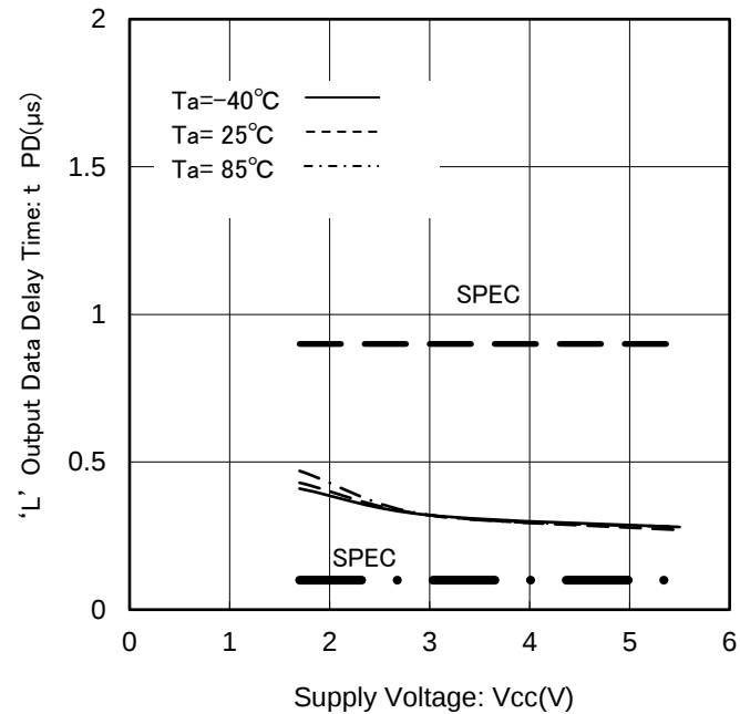
Figure 22. 'L' Output Data Delay Time vs Supply Voltage
