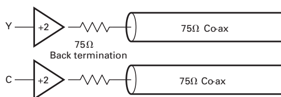
Dual amplifier S - video driver
