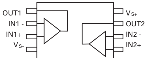
ZXFB204 Dual
