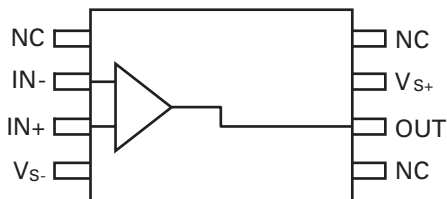
ZXFB202N8 Single
