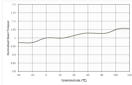
Figure 2. Normalized RESET Timeout Period vs Temperature
