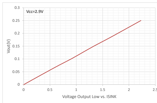
Figure 4. Voltage Output Low vs I_{SINK} (TPV809)
