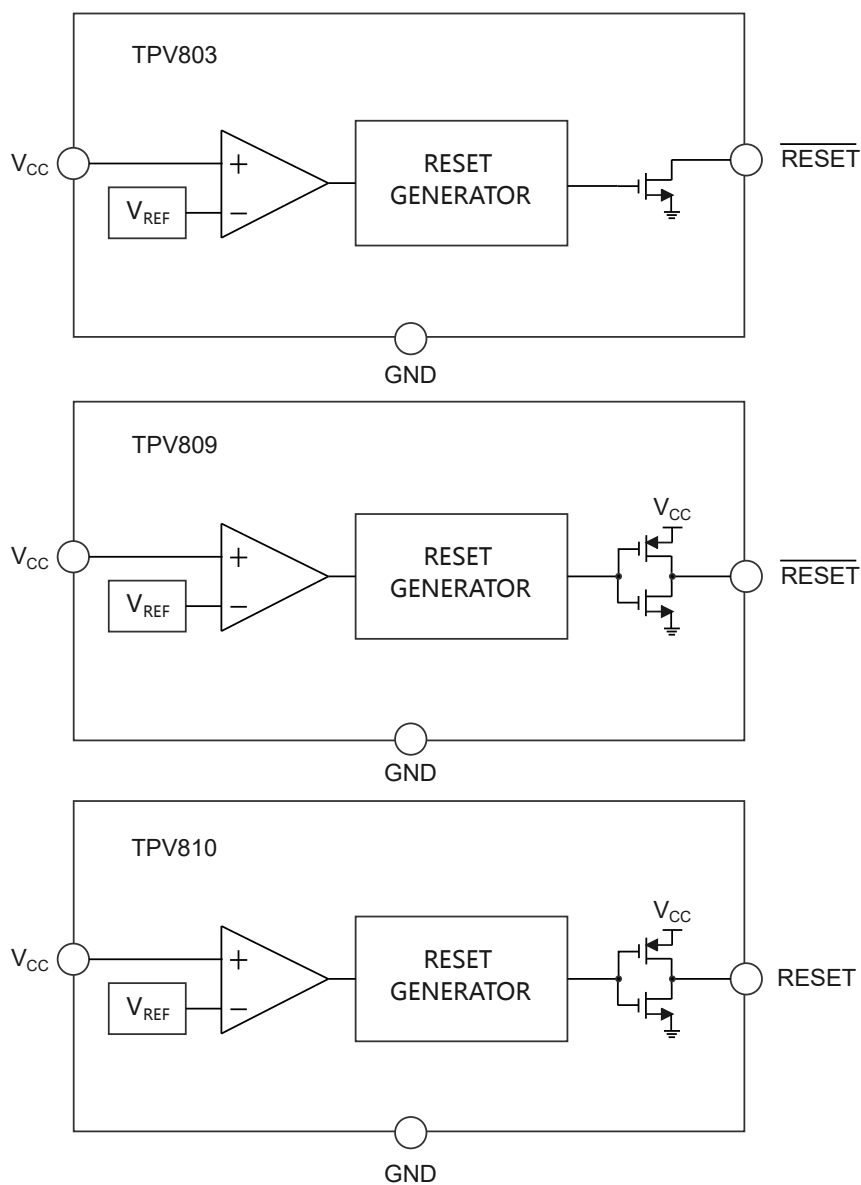
Figure 7. Functional Block Diagram
