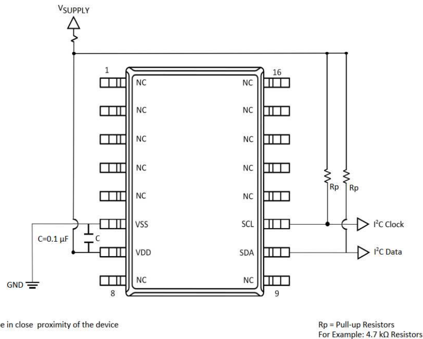
SM9541 + Family Applications Circuit
