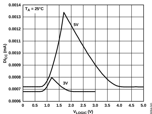
Figure 24. D_{Logic} vs. Logic Input Voltage
