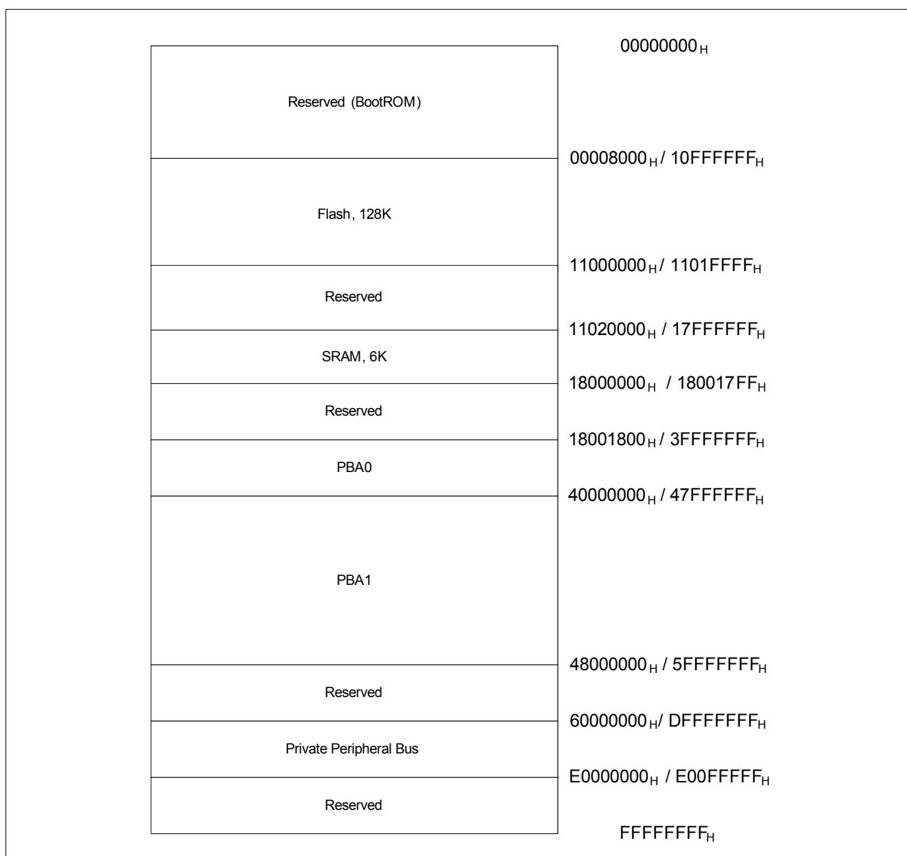
Figure 14 TLE9869QXA20 Memory Map
