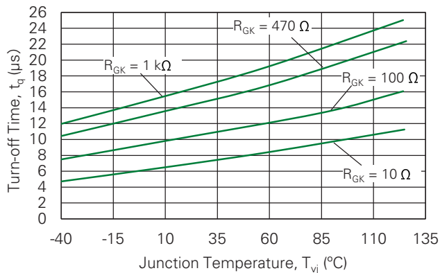
Fig. 10-2. Typical DC Turn-off Time with R_{GK} vs. Junction Temperature for S8X8xS3
