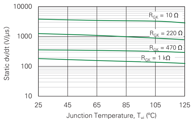
Fig. 9-2. Typical DC Static dv/dt with R_{GK} vs. Junction Temperature for S8X8xS3
