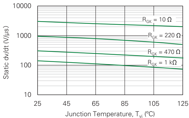
Fig. 9-1. Typical DC Static dv/dt with R_{GK} vs. Junction Temperature for S6X8xS3
