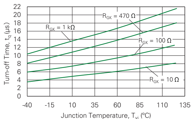
Fig. 10-1. Typical DC Turn-off Time with R_{GK} vs. Junction Temperature for S6X8xS3
