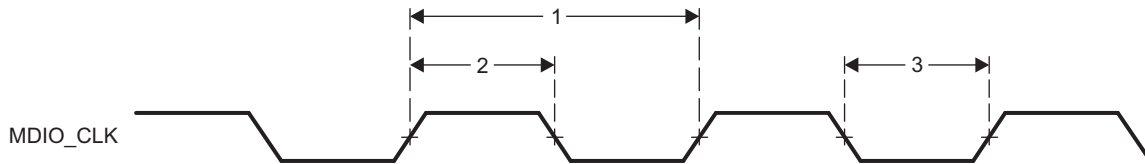
Figure 5-124. PRU-ICSS MDIO_CLK Timing
