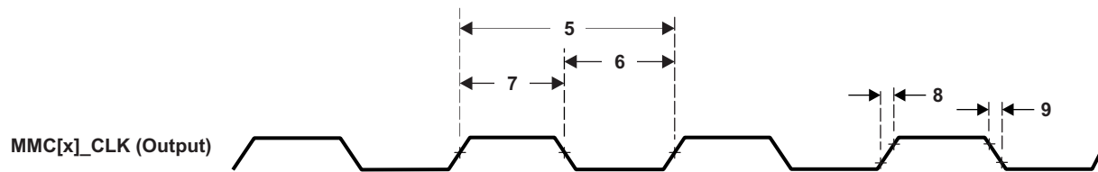
Figure 5-132. MMC[x]_CLK Timing
