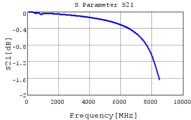
GCM1885C2A681JA16 S21 DCOV, 25degC
