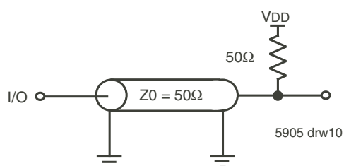
Figure 6. AC Termination
