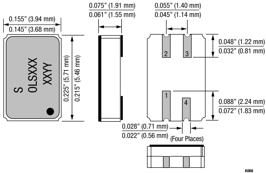
Figure 6. OLS049 Package Dimensions
