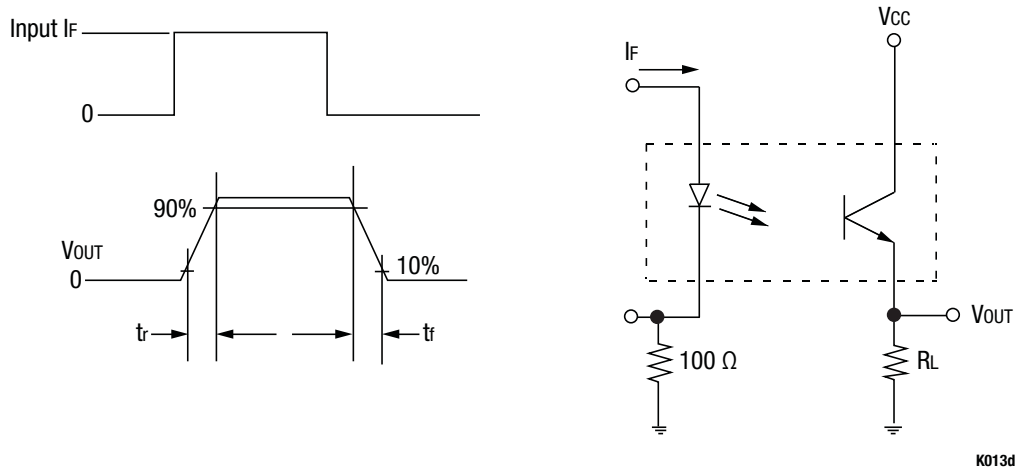
Figure 5. OLS049 Switching Test Circuit
