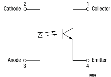
Figure 1. OLS049 Block Diagram
