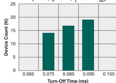
Typical Turn-Off Time (N=50, I_F=5\text{mA} , I_L=350\text{mA}_{DC} )
