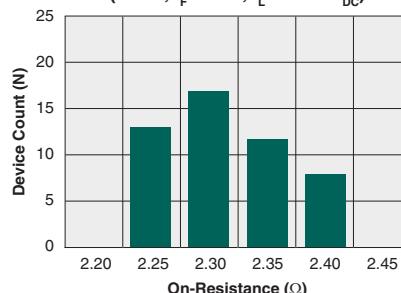
Typical On-Resistance Distribution (N=50, I_F=5\text{mA} , I_L=350\text{mA}_{DC} )
