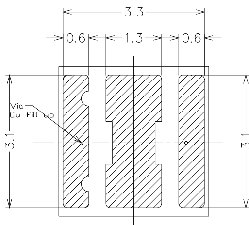
Solder pad design
