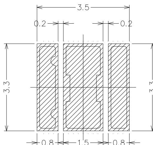
Soldering patterns
