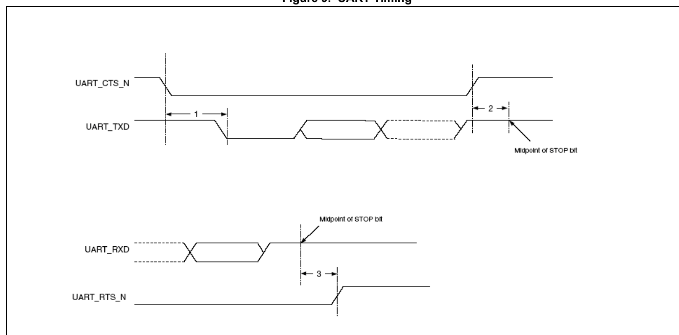
Figure 9. UART Timing
