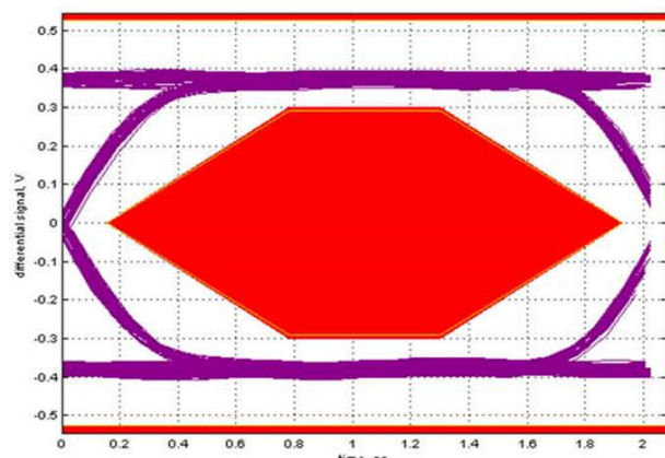
Figure 5-3. Typical High-Speed (480 Mbps) Eye-Diagram through ISOUSB211-Q1
