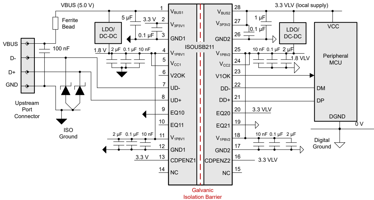
Figure 8-7. Using ISOUSB211-Q1 with 1.8-V supplied with External Regulators
