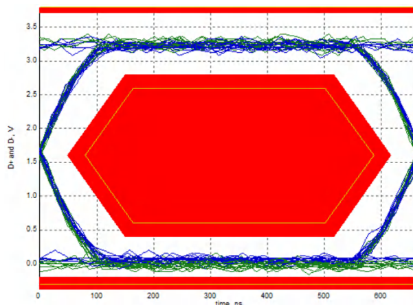
Figure 5-5. Typical Low-Speed (1.5 Mbps) Eye-Diagram through ISOUSB211-Q1
