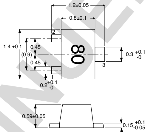
PIN CONNECTIONS
