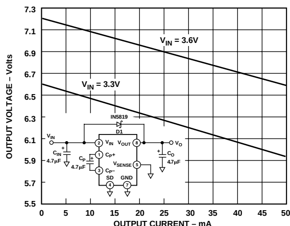
Figure 18. Maximum Unregulated Output Voltage
