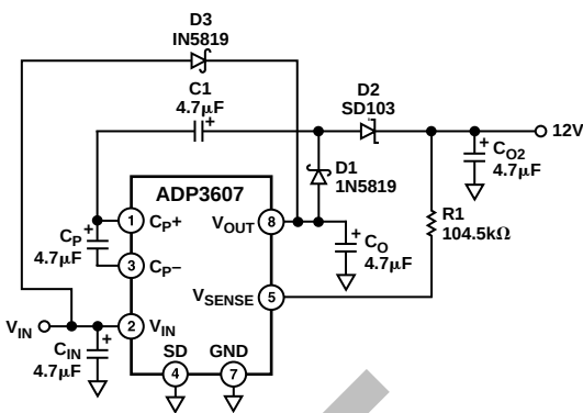
Figure 20. Regulated 12 V from a 5 V Input
