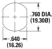
Panel Mounting
