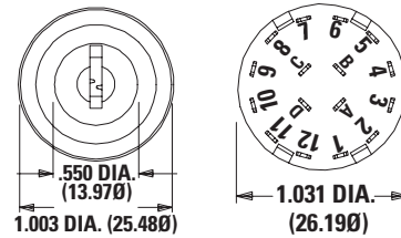
Panel Mounting
