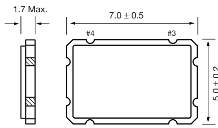
Figure 1) CSM-8 – Side and Top view
